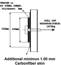
SECTION B-B
