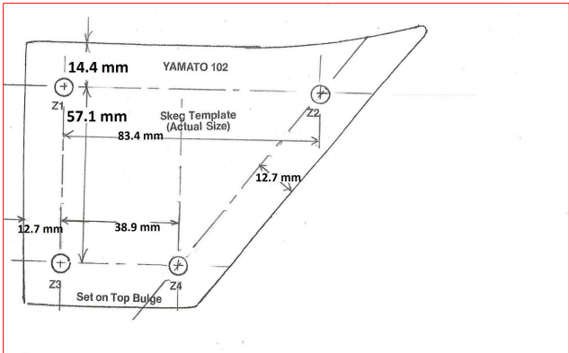
↑ Additional measurements for Skeg
