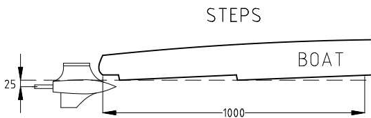
HYDROPLANE PROPELLER SHAFT HEIGHT MEASUREMENTS
