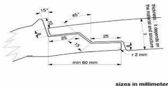
Main hatch flange minimum dimensions
