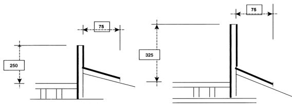
Sections B
